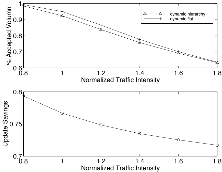
Figure 3: Percent routed volume comparison (top) and update savings (bottom) achieved by the effective resistance hierarchical routing.
